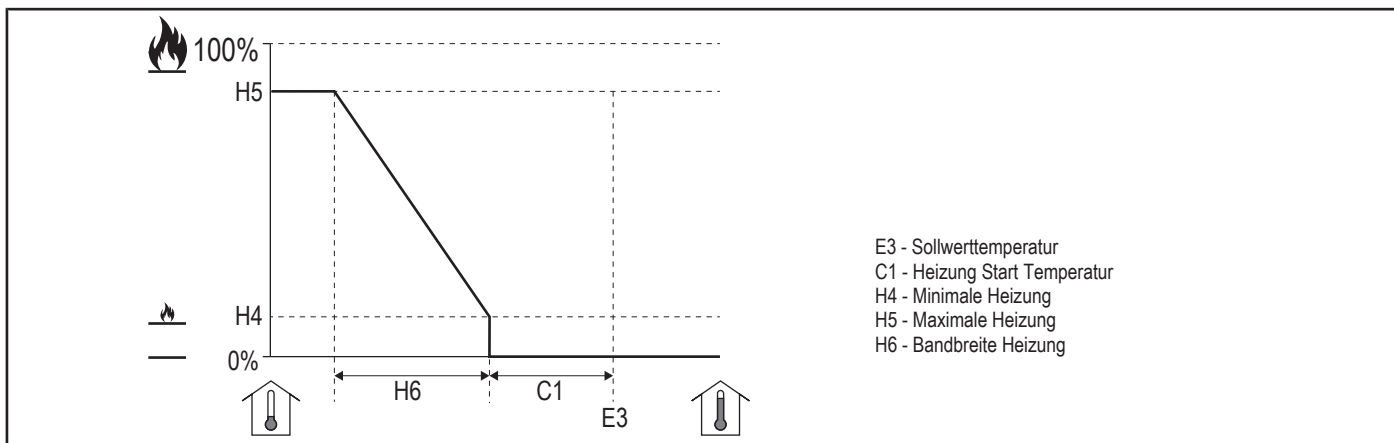
Abb. 7: Heizung [0 - 10 V]
