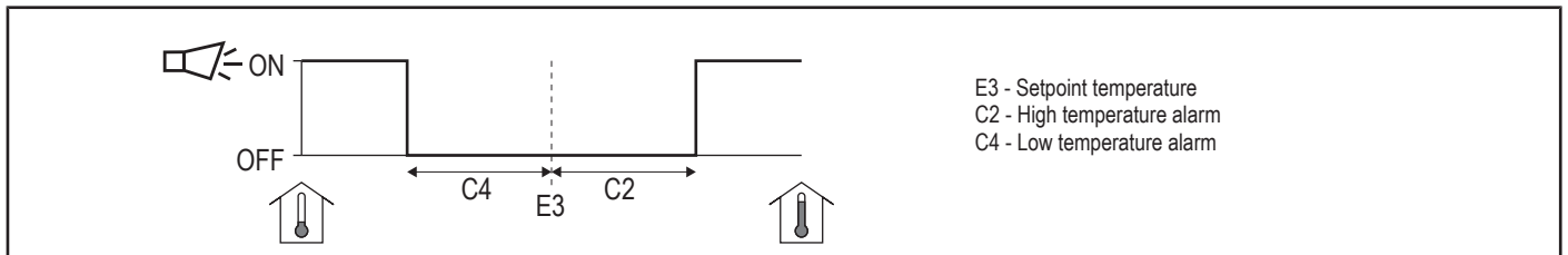
Illustration 8: Temperature alarms
