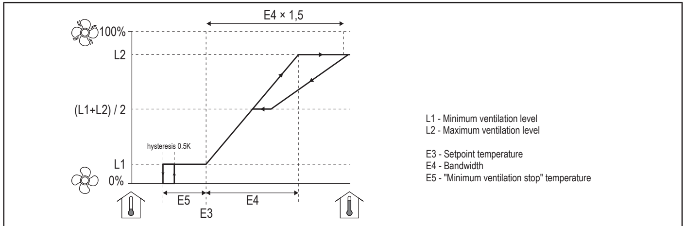
Illustration 4: Bandwidth compensation
