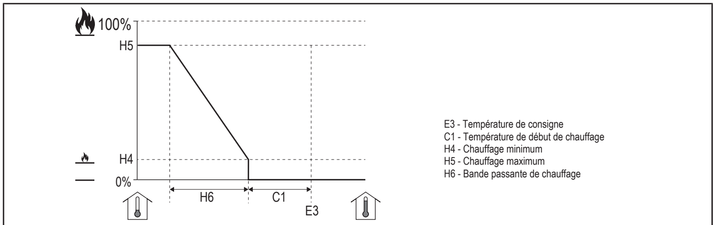
Fig. 7: Chauffage [0 - 10 V]
