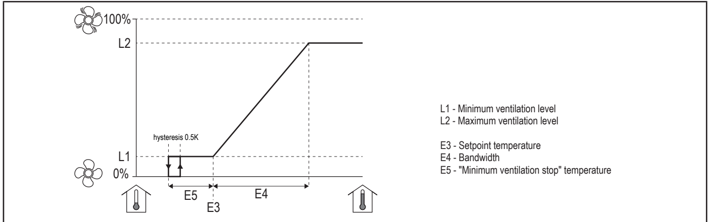
Illustration 2: Ventilation level
