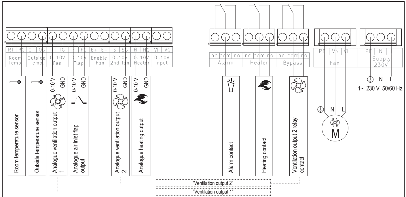
Illustration 1: Wiring Diagram
