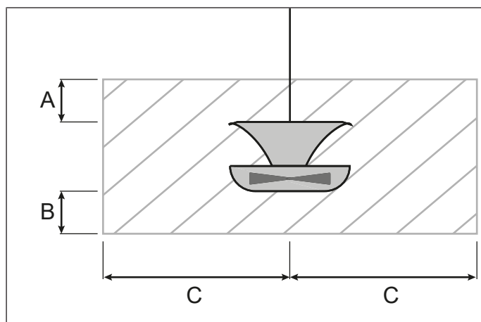
Fig. 5: Zone sans obstacle V-FloFan
