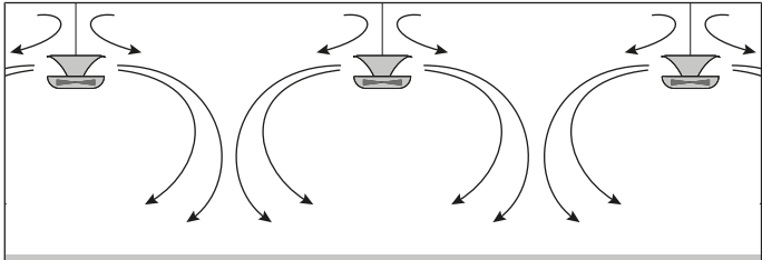
Illustration 2: VFloFan operating principle
