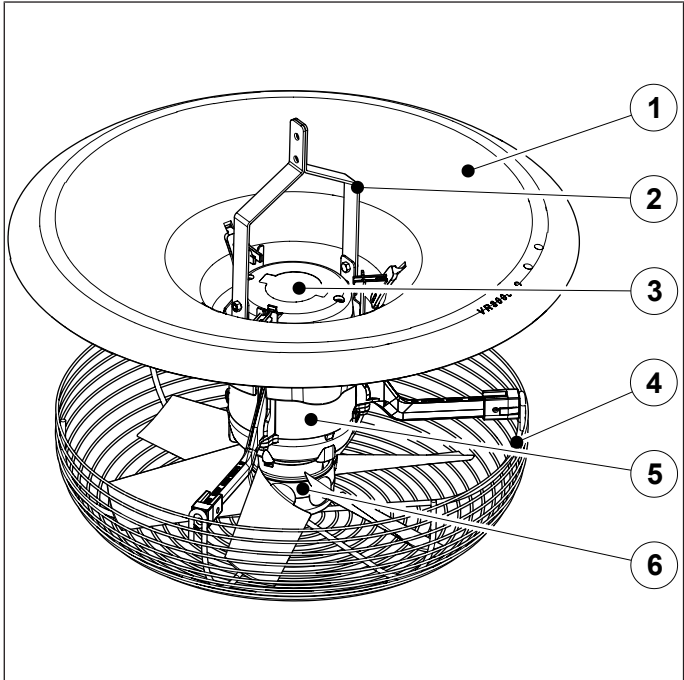
Illustration 1: V-FloFan overview
