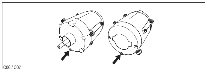
Illustration 5: Condensate drain hole locations
